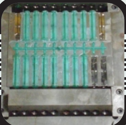
Industrial Syringe Plunger Mould
